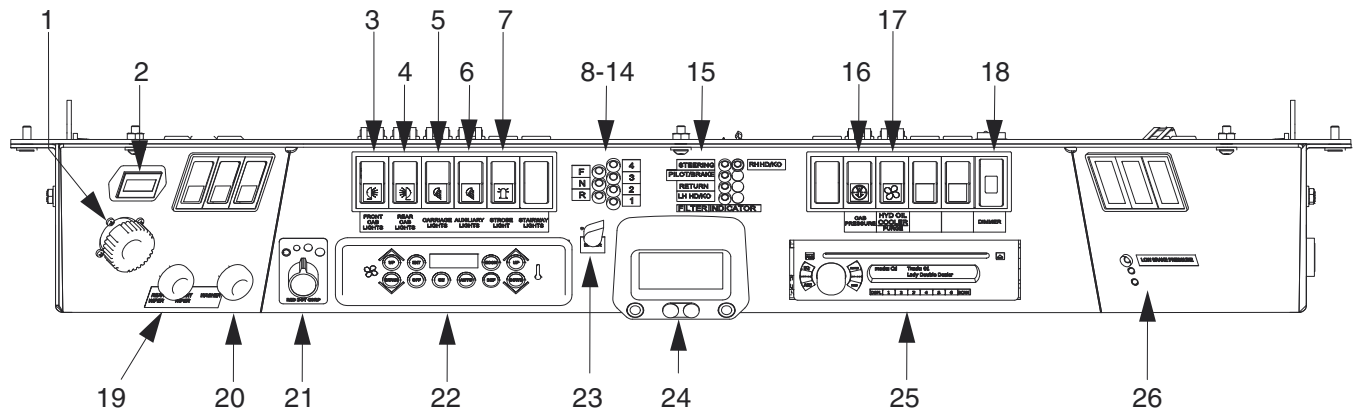
Figure 2-3-1 Overhead Console
