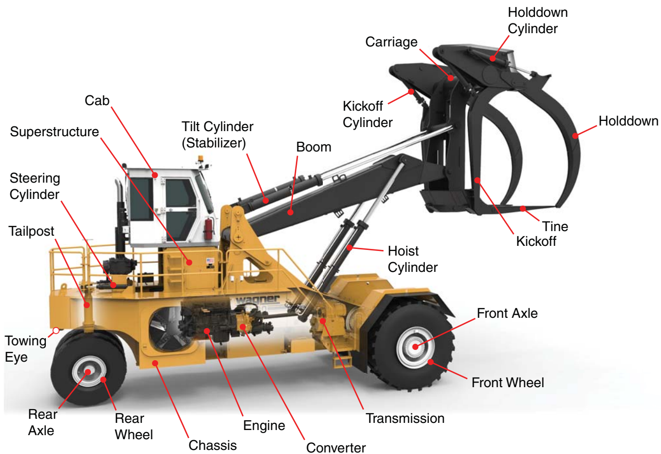
Figure 1-3-2 Terminology (Model L90 Shown for Reference)
