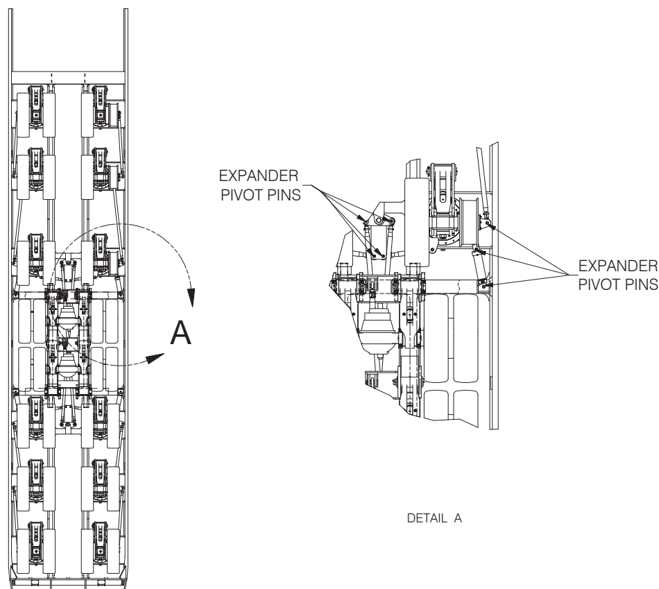
Figure 2 - Locations of Typical Expander Pin System (At the each end of Steering Cylinders.)
