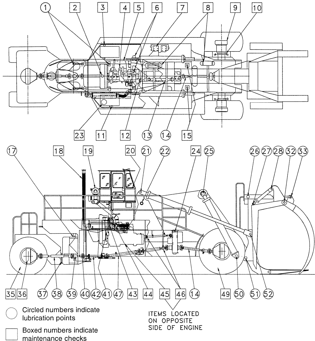
L490 Maintenance and Lubrication Chart
