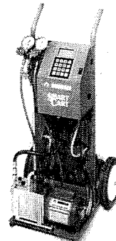
b.) ALL PURPOSE CHARGING STATION INCLUDES AUTOMATIC EVACUATION, OIL INJECTION, RECHARGING, ELECTRONIC CONTROLS TO ADJUST VACUUM PUMPING TIME AND LEAK DETECTION
