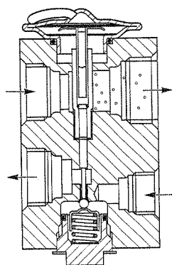
PRESSURE CONTROLLED BLOCK TYPE TXV
