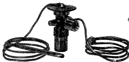
TYPICAL PRESSURE CONTROLLED TXV (EXTERNALLY EQUALIZED)
