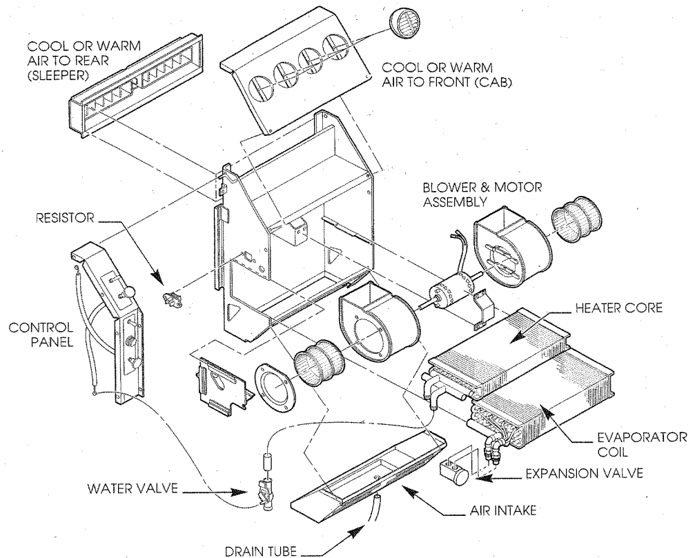
HVAC COMBINATION UNIT
