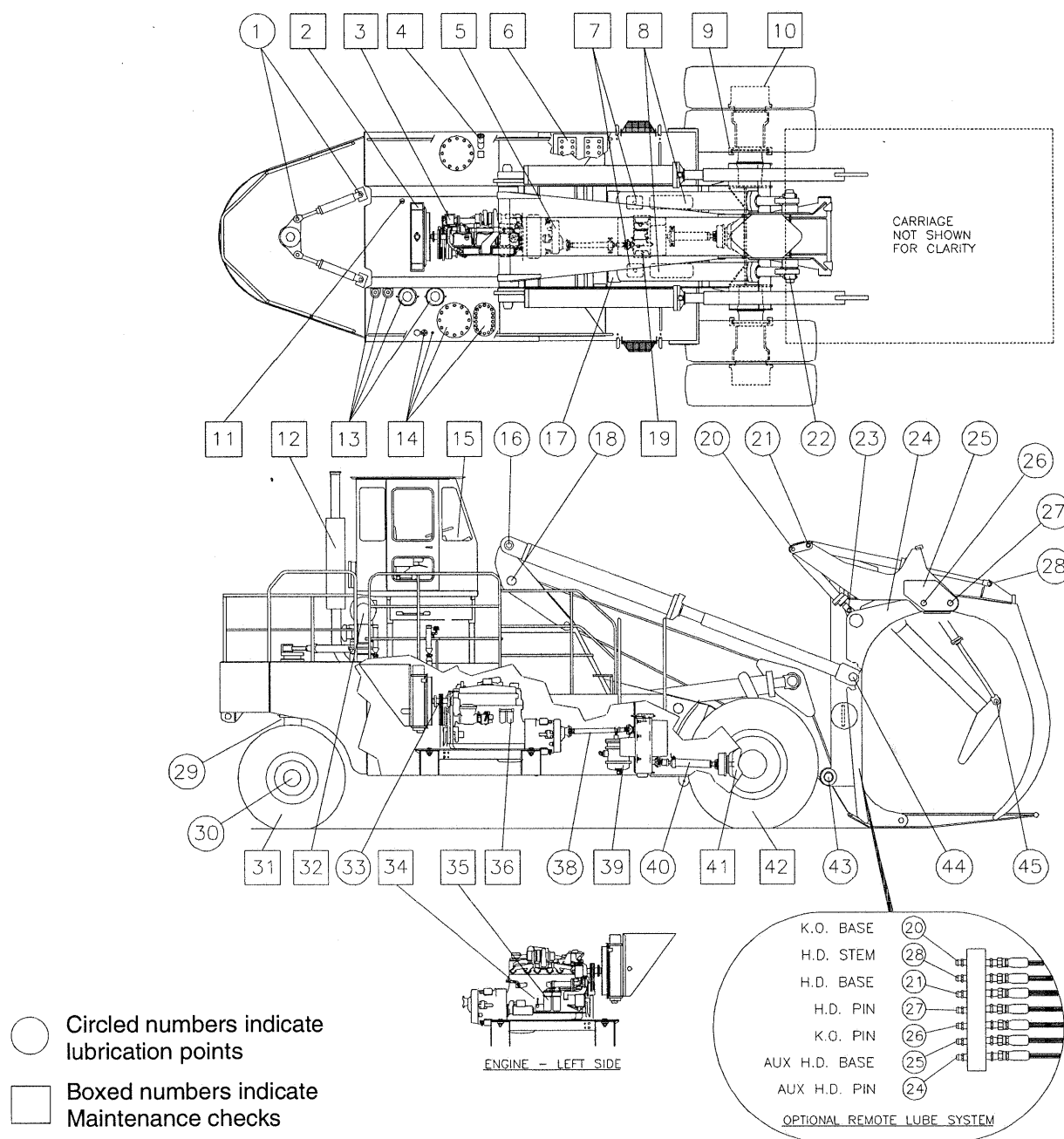
Fig. 1 L80F Maintenance and Lubrication Chart
