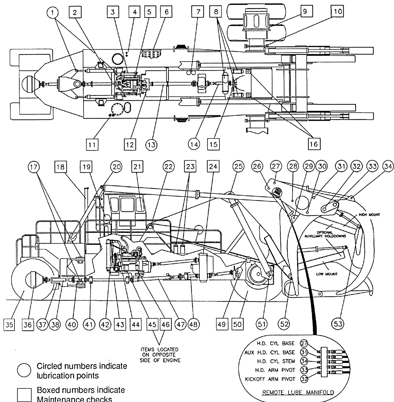
Fig. 1 L-4130 Maintenance and Lubrication Chart
