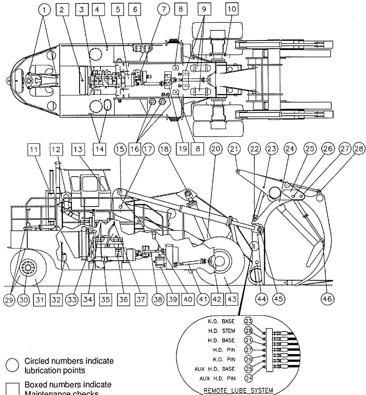
Fig. 1 L-4100H Maintenance and Lubrication Chart
