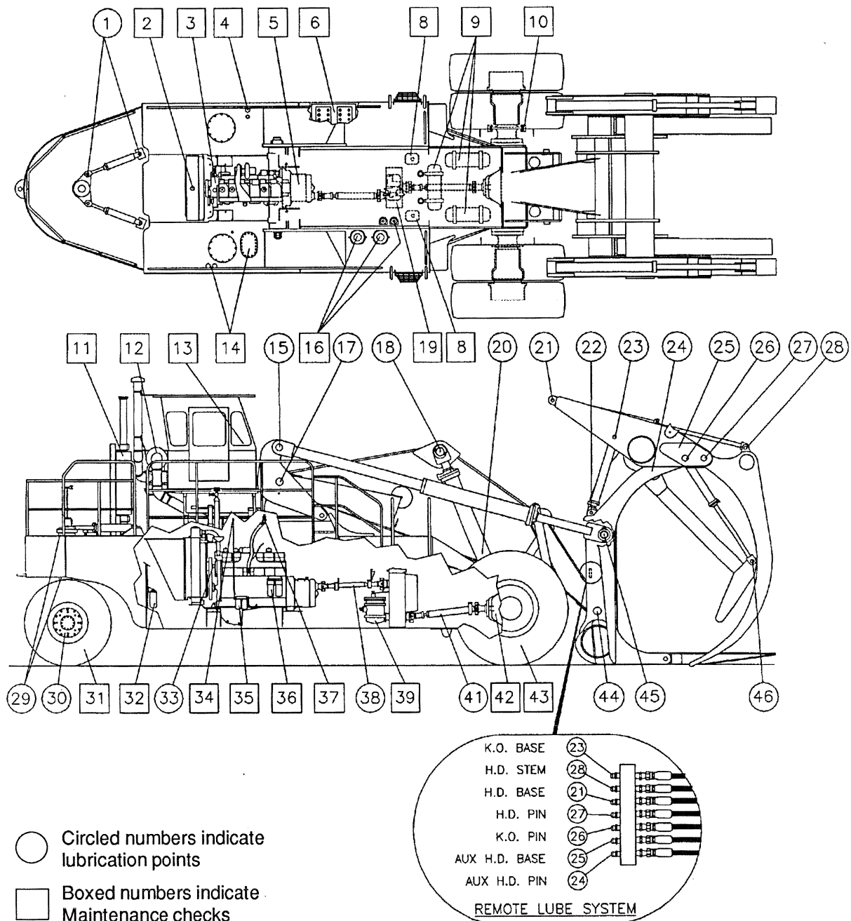
Fig. 1 L-100 Maintenance and Lubrication Chart
