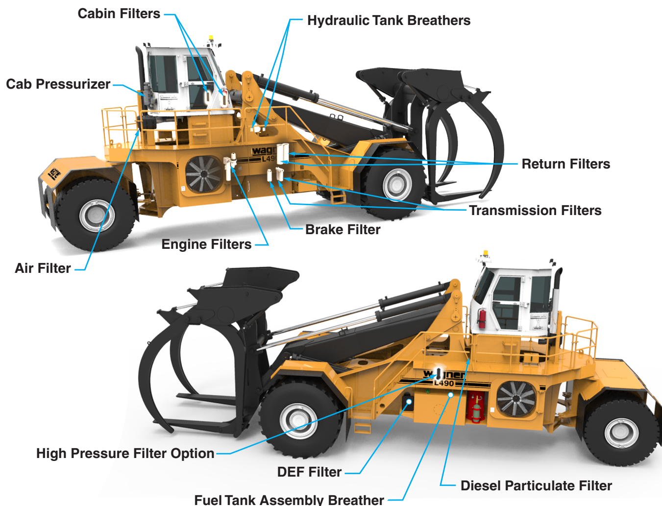
1 Filter Arrangement
