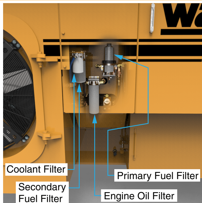
6 Engine Filters
