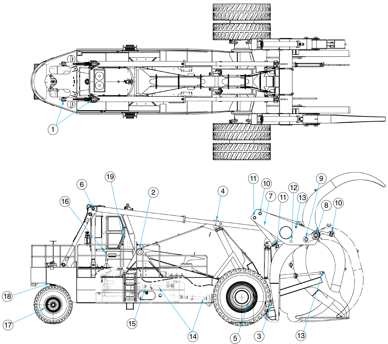
Figure 1 Lubrication Points
