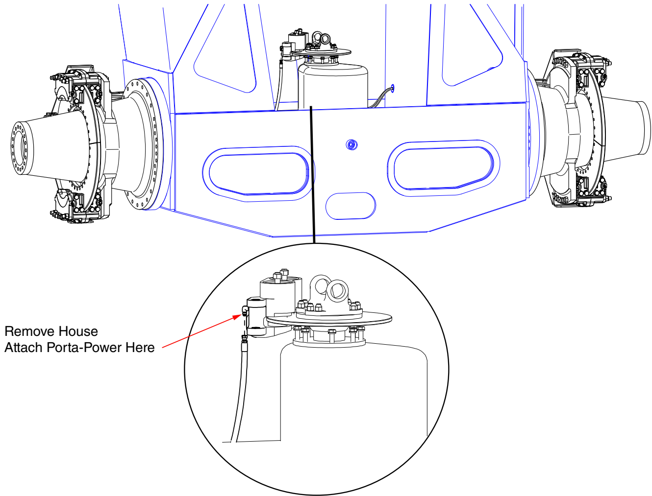
Figure 2 Connect Porta-Power
