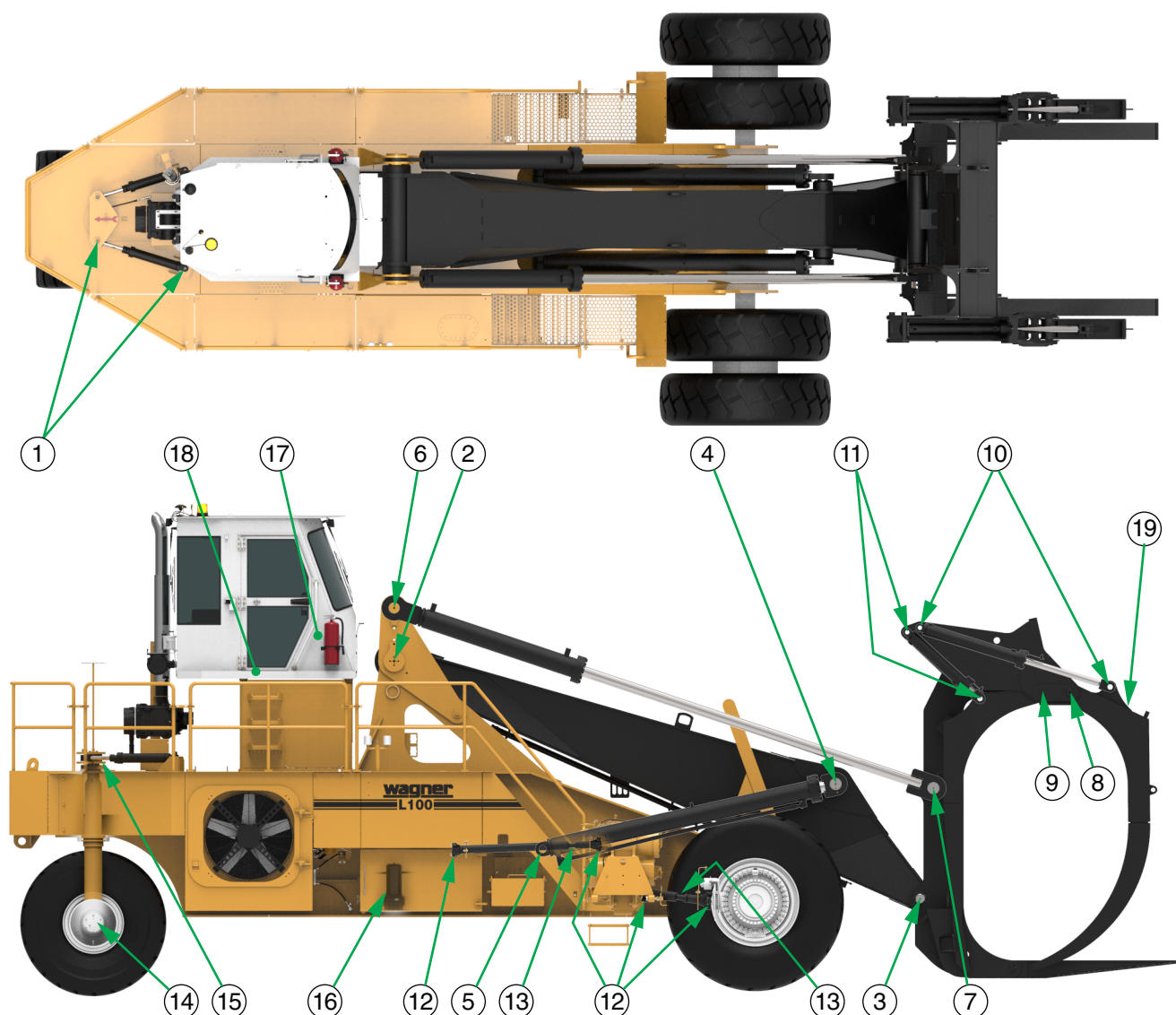
Figure 1 Lubrication Points
