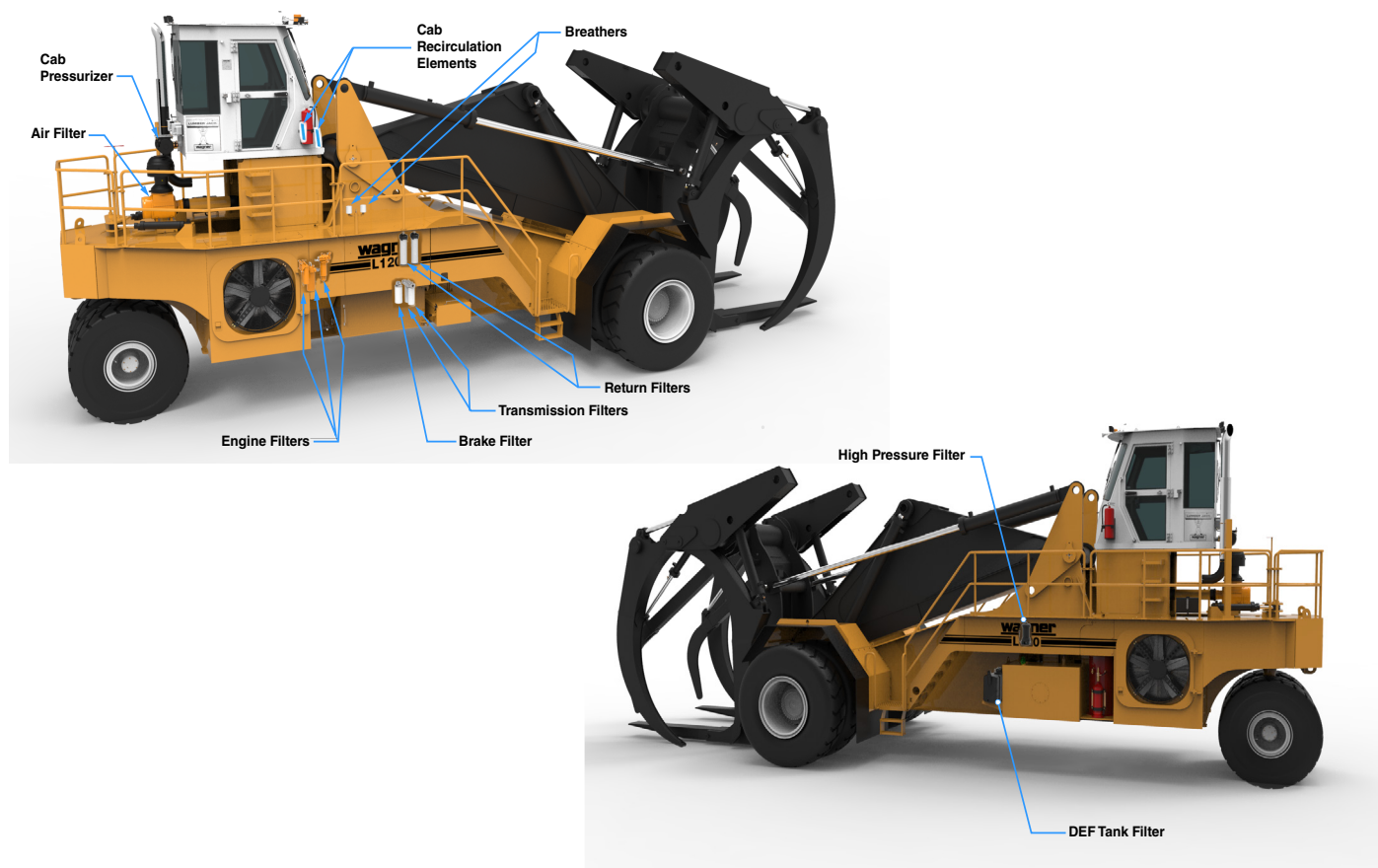
Figure 5-5-1 Filter Arrangement
