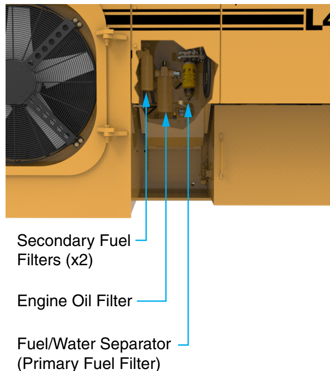
Figure 5-5-6 Engine Filters
