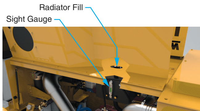
Figure 1 Surge Tank Location
