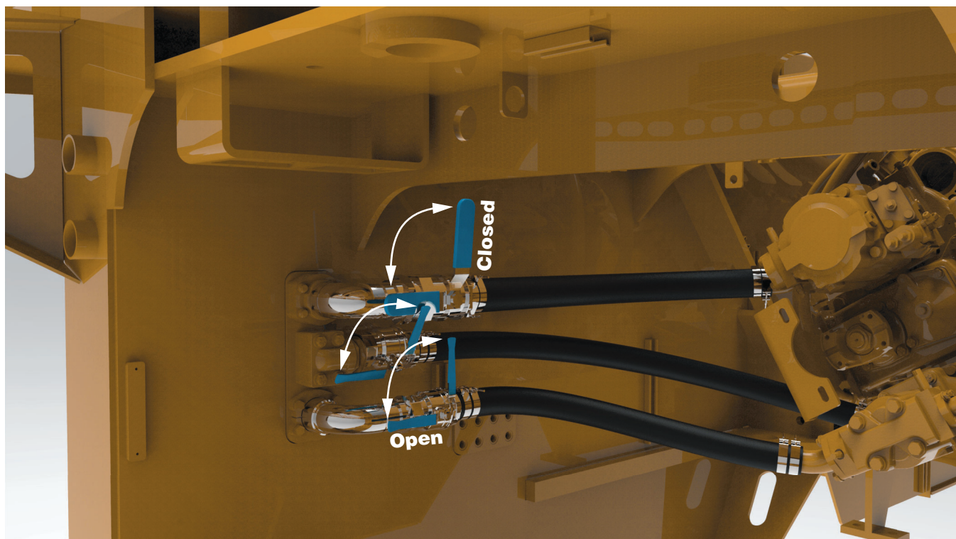
Figure 1 Shutoff Ball Valves (components removed from view for visibility)
