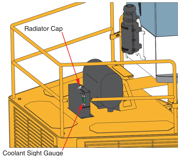
Figure 1 Radiator Cap and Coolant Sight Gauge, L460
