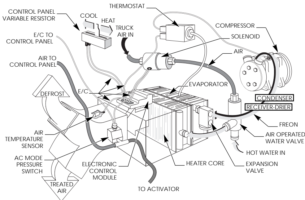
Figure 10-3 The CTC II system is shown in this drawing.
