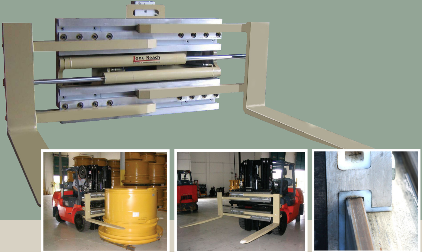
Easily replaced polymer wear strips
