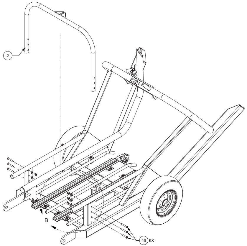
BALE GUIDE INSTALLATION
