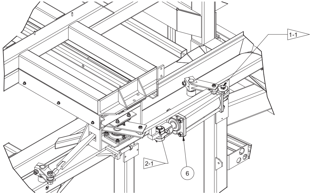
DETAIL D
