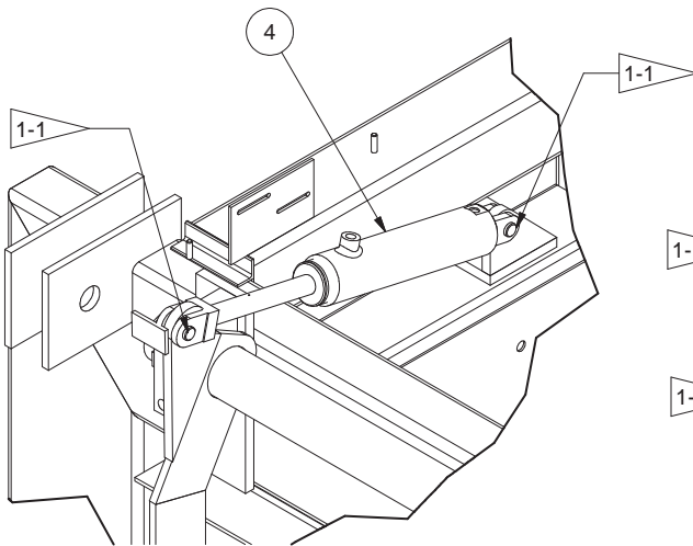
DETAIL H
