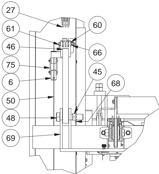
DETAIL AD
