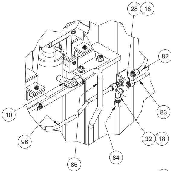
DETAIL E
