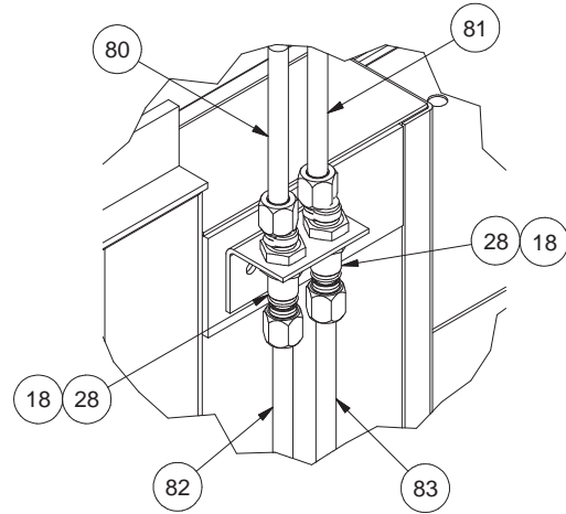
DETAIL D
