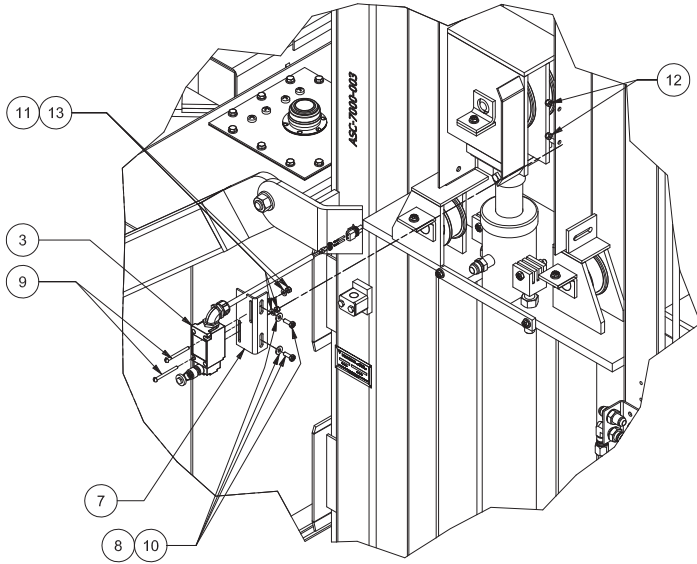
DETAIL E
