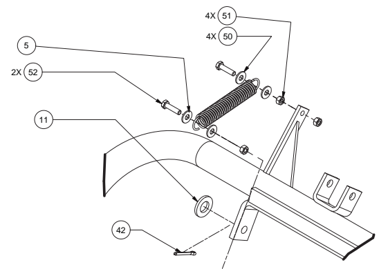
DETAIL C
