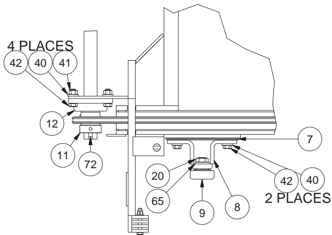
DETAIL AM
