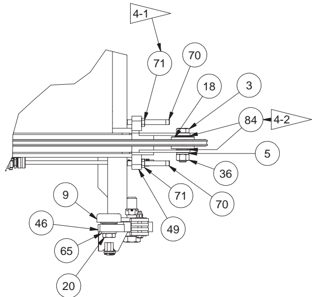
DETAIL AT
