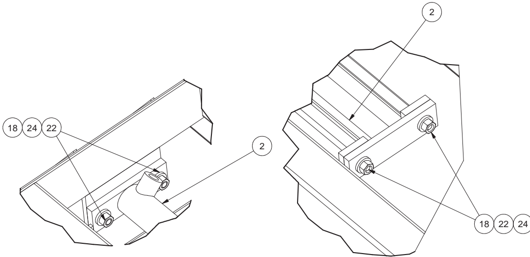
DETAIL F
