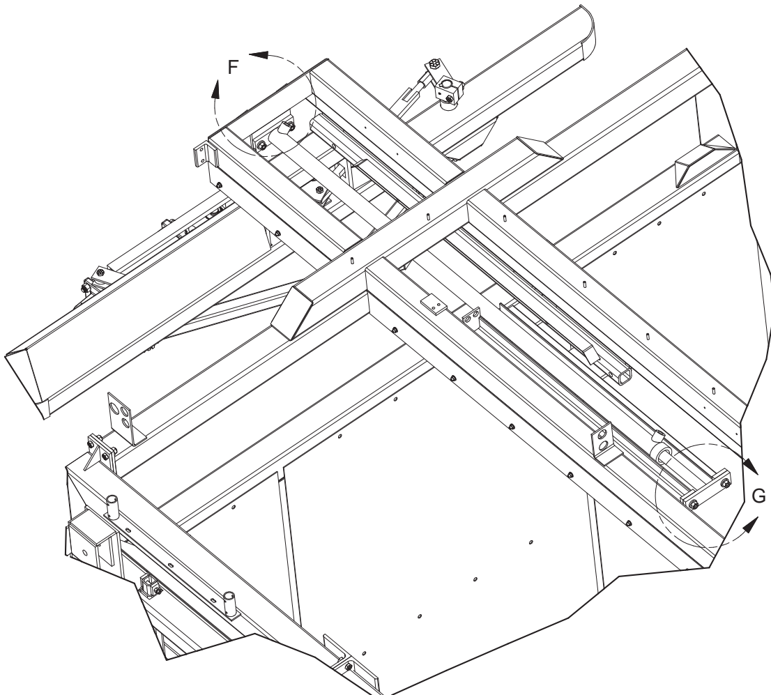
DETAIL E
