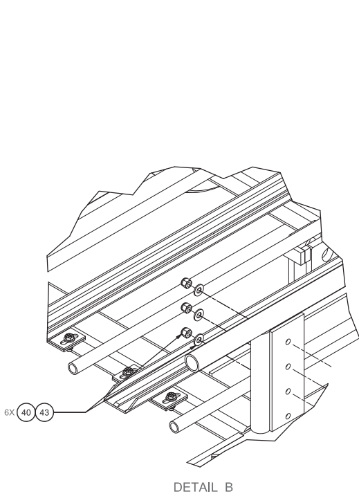
DETAIL B
