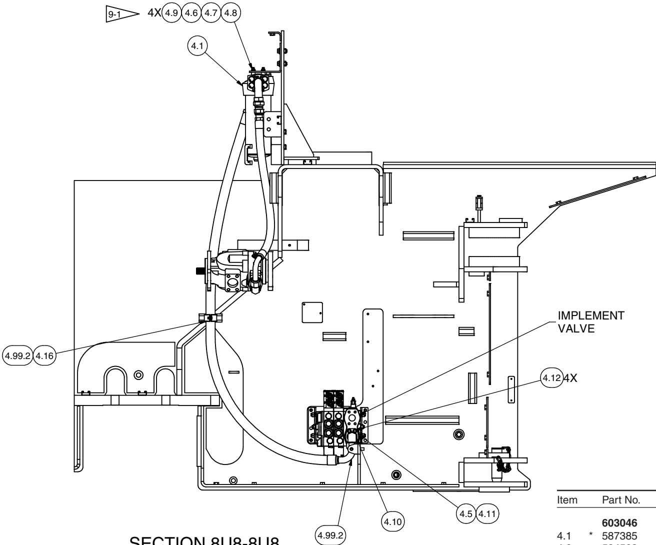
SECTION 8U8-8U8 LH SIDE
