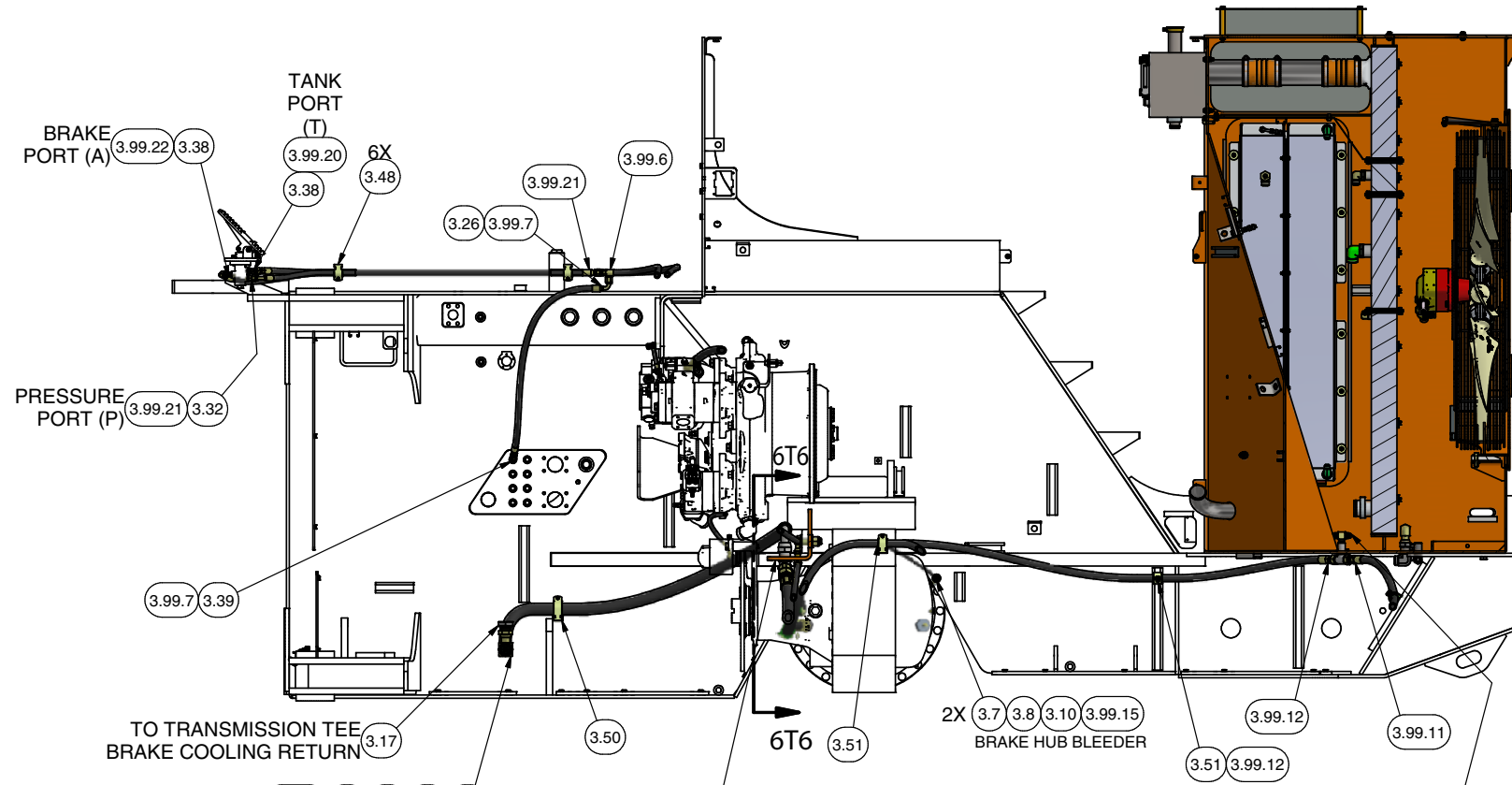
SECTION 6V5-6V5 RH INTERIOR VIEW SEE COOLING PACKAGE FOR CONTINUATION OF PLUMBING
