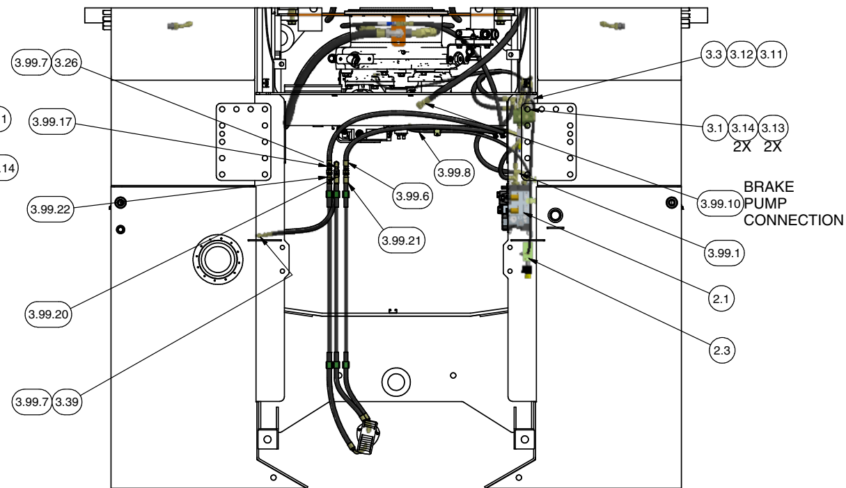
SECTION 6W5-6W5 FROM TOP
