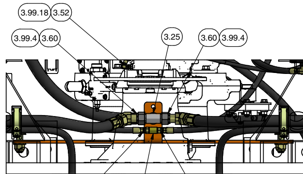
SECTION 6T6-6T6
