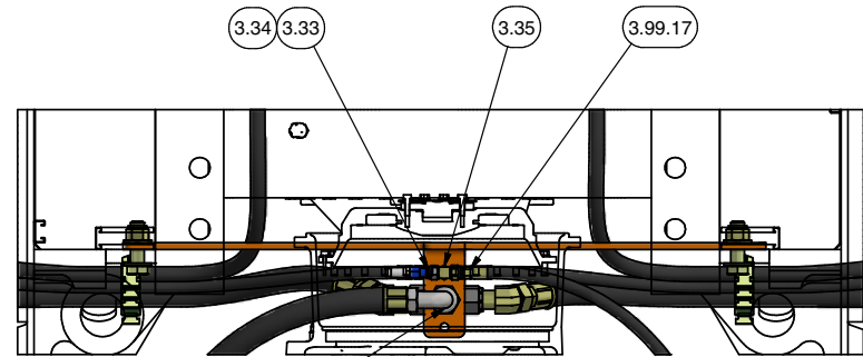
VIEW 6S6-6S6 BRAKE PLUMBING DISTRIBUTION
