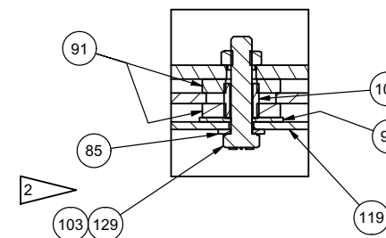
SECTION 3D3-3D3 6 PLACES - SCANIA
