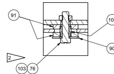
SECTION 3D3-3D3 20 PLACES - CUMMINS 14 PLACES - SCANIA
