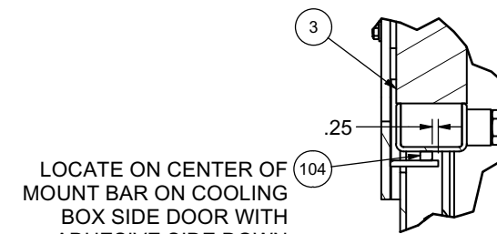
DETAIL 4M4 TYP. BOTH SIDES
