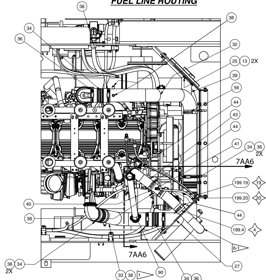
SECTION 6T2-6T2 CAC PLUMBING & JACKET WATER (HOT) INSTL COMPONENTS REMOVED FOR CLARITY
