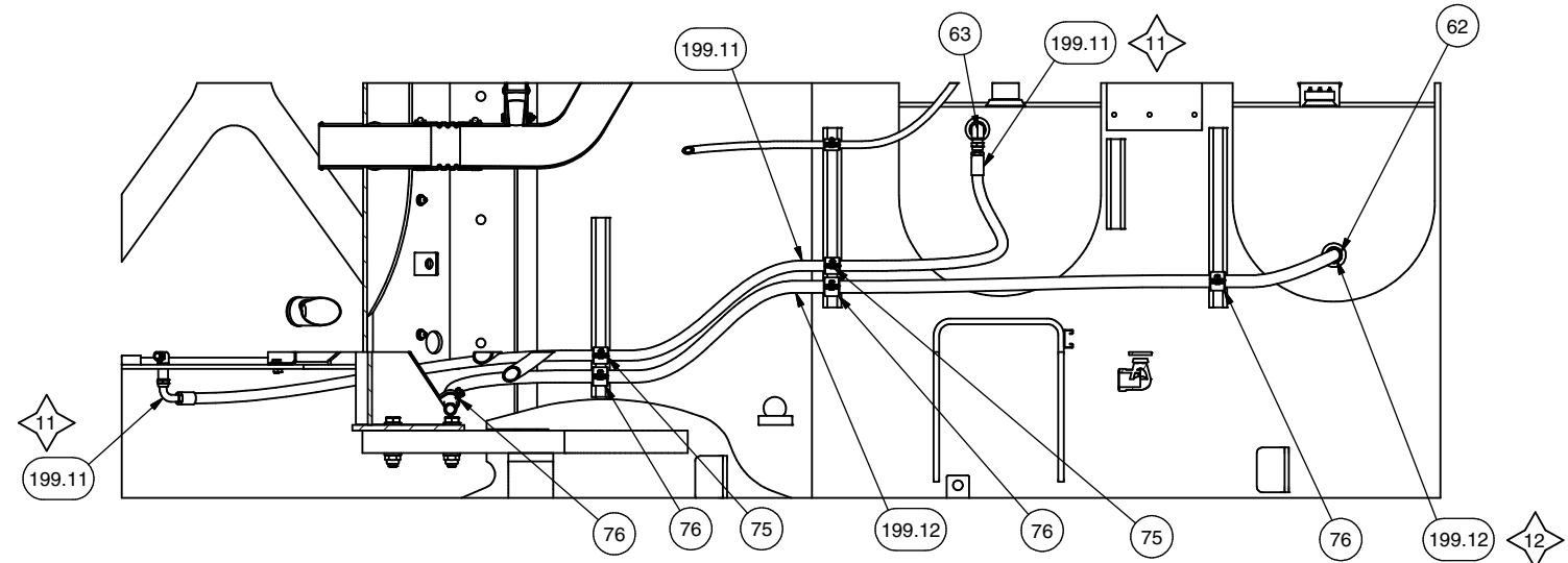
SECTION 6U6-6U6 FUEL LINE ROUTING
