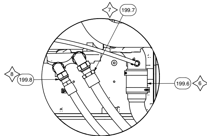
DETAIL 4M4 OIL FILTER LINES (ENGINE SIDE)
