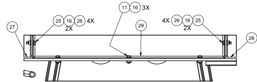
DETAIL 3H3
