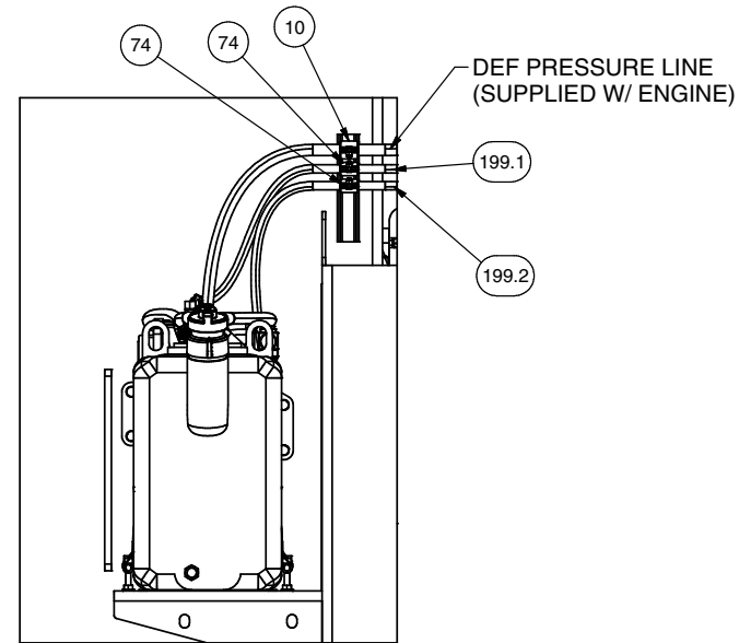
VIEW 7Z2-7Z2 DEF TANK INSTL/PLUMBING
