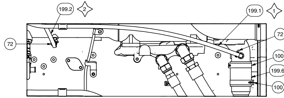
DETAIL 7Y4 DEF COOLANT ENGINE CONNECTIONS
