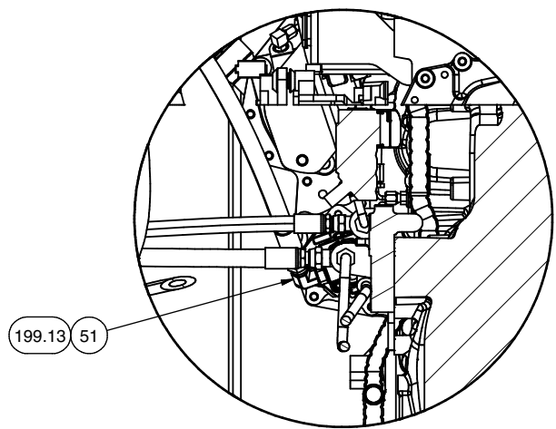
DETAIL 6S6 FUEL FILTER PLUMBING (ENGINE SIDE)
