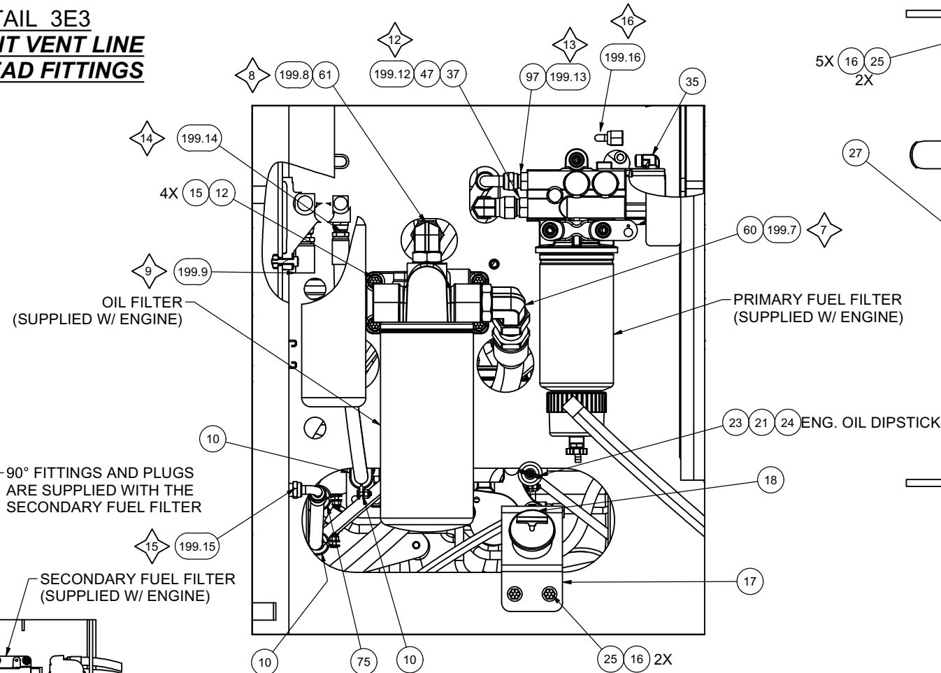
DETAIL 3G2 OIL FILTER/ FUEL FILTER INSTL
