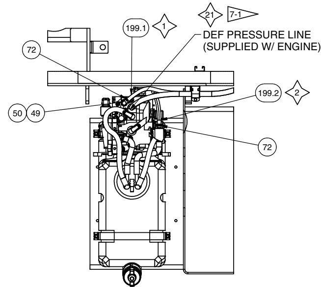
DETAIL 7Y4 DEF COOLANT ENGINE CONNECTIONS
