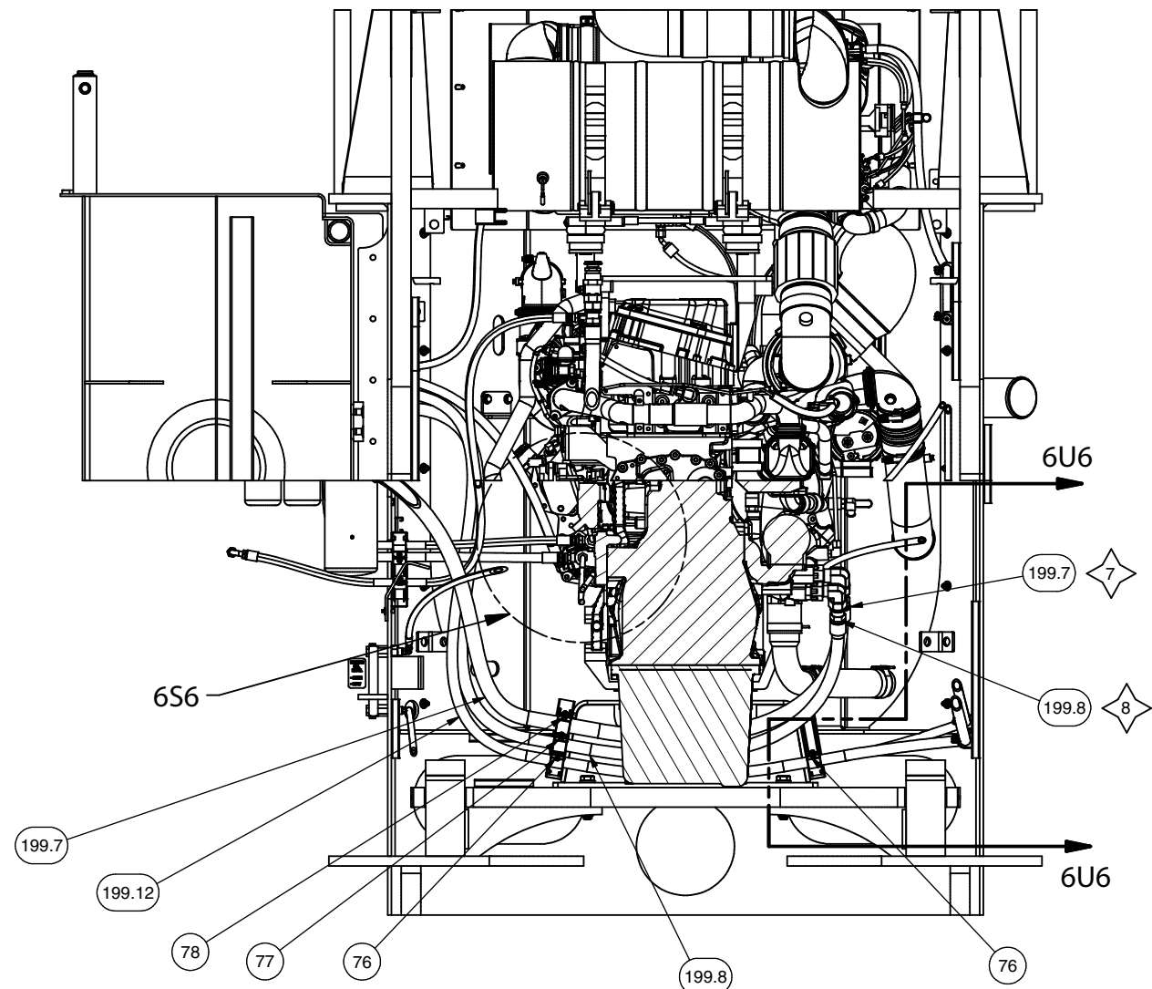
SECTION 6R2-6R2 PLUMBING INSTL ITEMS REMOVED FOR CLARITY
