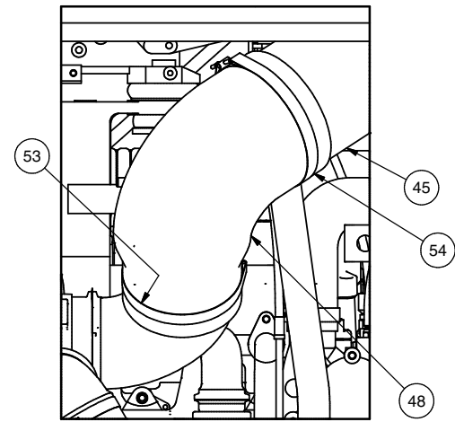
DETAIL 4P4 AIR CLEANER INSTL COMPONENTS REMOVED FOR CLARITY
