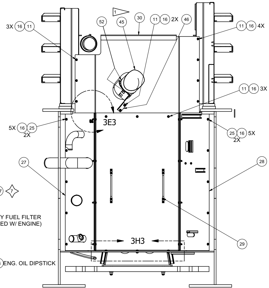
SECTION 3J2-3J2 BULKHEAD/ISOLATION PLATE INSTL VIEW ROTATED 90°
