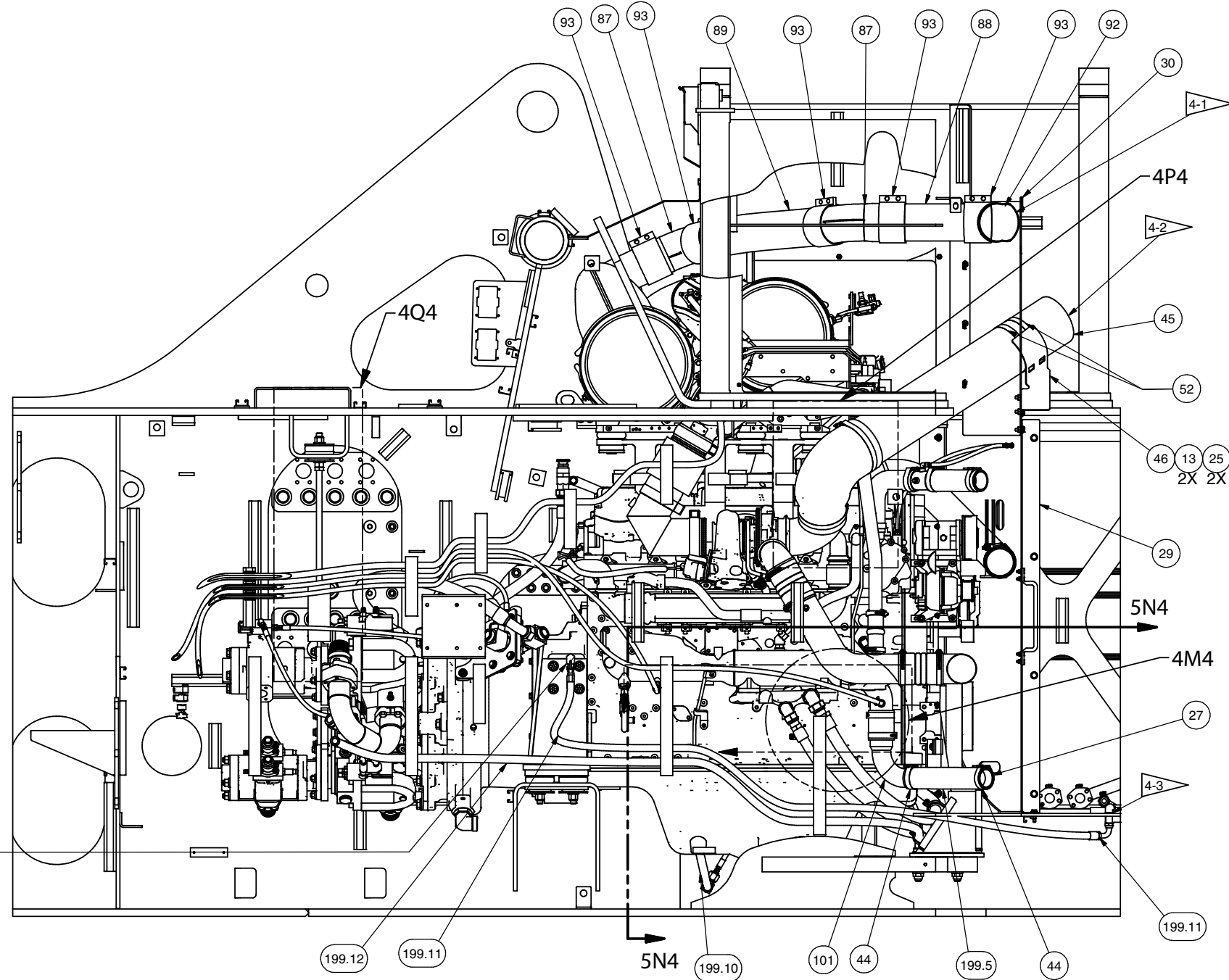
SECTION 4K2-4K2 COMPONENTS REMOVED FOR CLARITY
