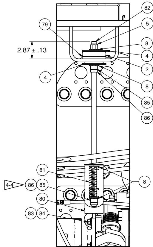
DETAIL 4Q4
