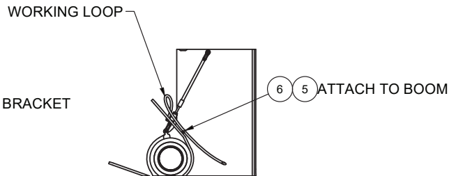
SECTION 23BF23-23BF23 BOOM-CARRIAGE POSITION SENSOR
