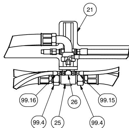
DETAIL 2D2 BRAKE PLUMBING DISTRIBUTION BRKT
