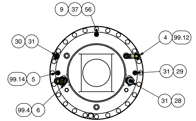
SECTION 2B2-2B2 RH BRAKE HUB PLUMBING
