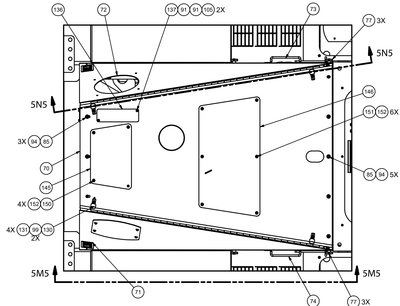
DETAIL 5L1 HOOD/PANEL INSTL
