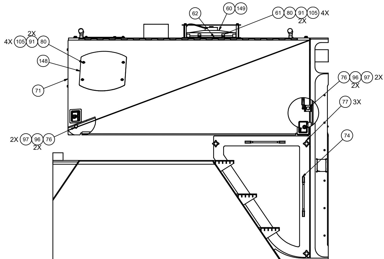
DETAIL 5L1 HOOD/PANEL INSTL
