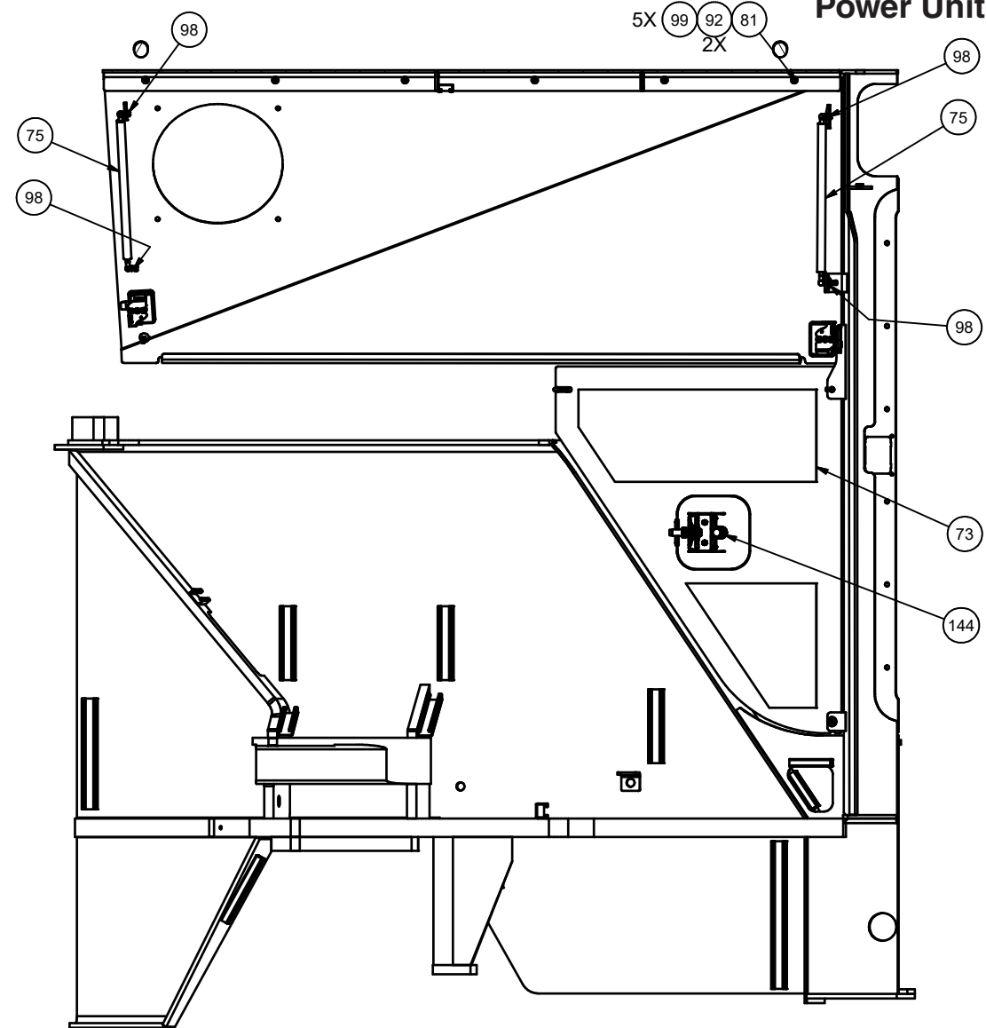
SECTION 5N5-5N5 TYP BOTH SIDES
