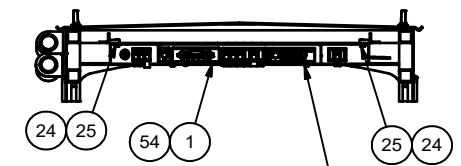
SECTION E-E
