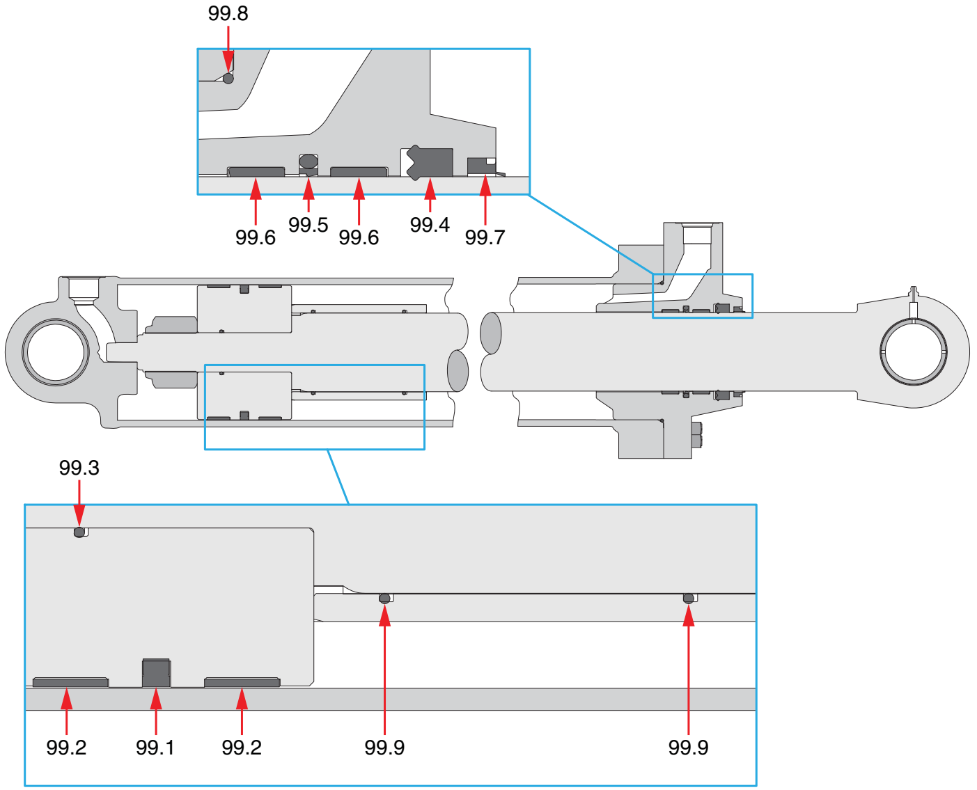
Packing Kit Detail
