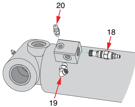
Cushion Relief Detail
