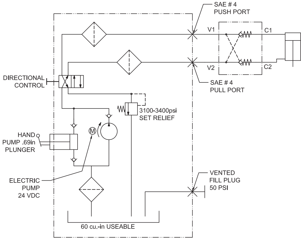
HYDRAULIC SCHEMATIC
