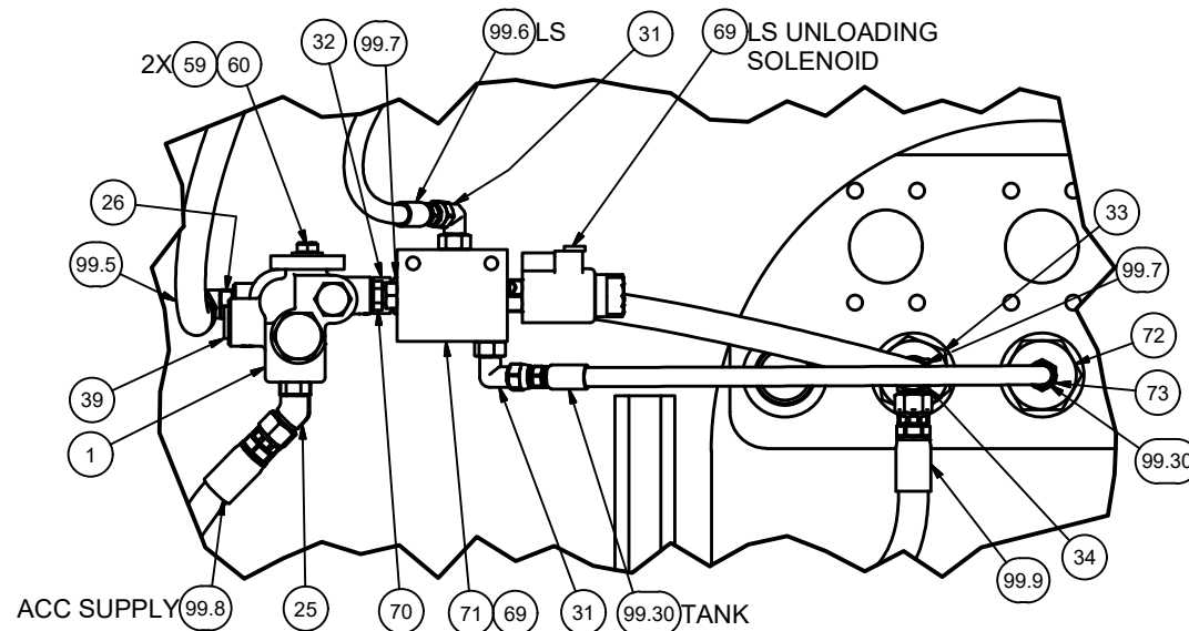
DETAIL 3F3 ACCUMULATOR CHARGE MANIFOLD & LS UNLOADING VAVLE
