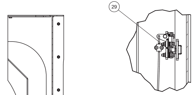
DETAIL 4N4
