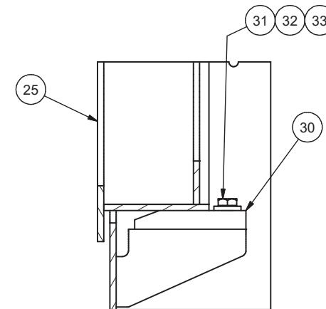
SECTION 4P4-4P4
