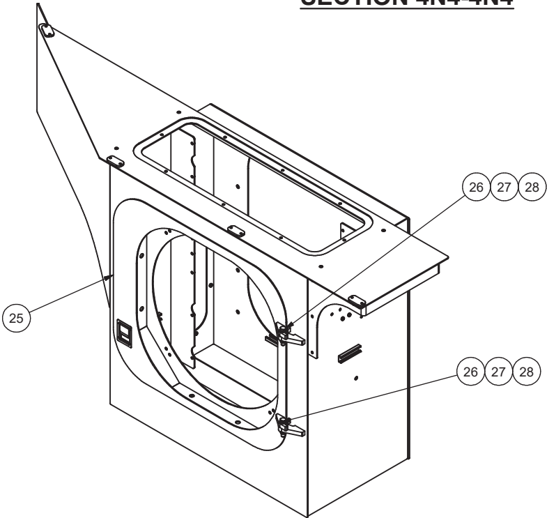
SECTION 4N4-4N4
