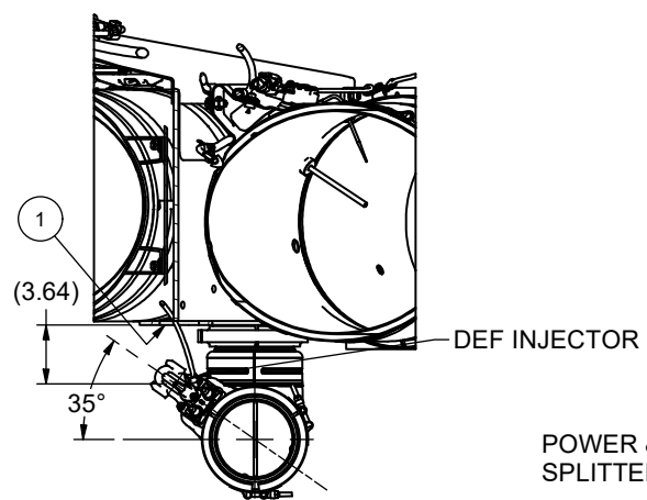
SECTION A-A VIEW ROTATED FOR CLARITY DRT ORIENTATION
