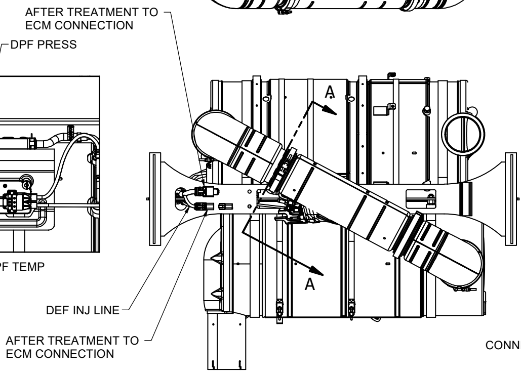
DETAIL B
