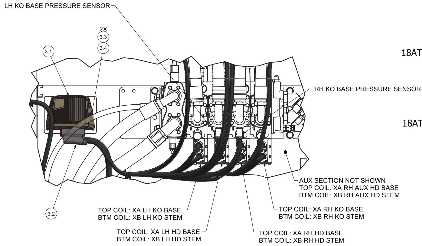
DETAIL 18AU18 CARRIAGE HEAD WIRING SOME PARTS REMOVED FOR CLARITY
