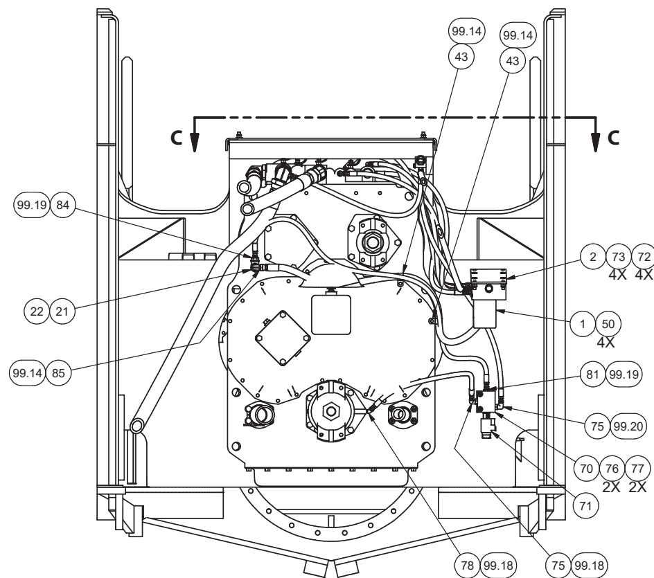
SECTION F-F SOME COMPONENTS REMOVED
