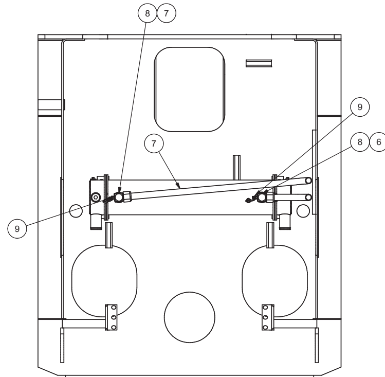
SECTION D-D VIEW ROTATE 90° TUBE & SHELL
