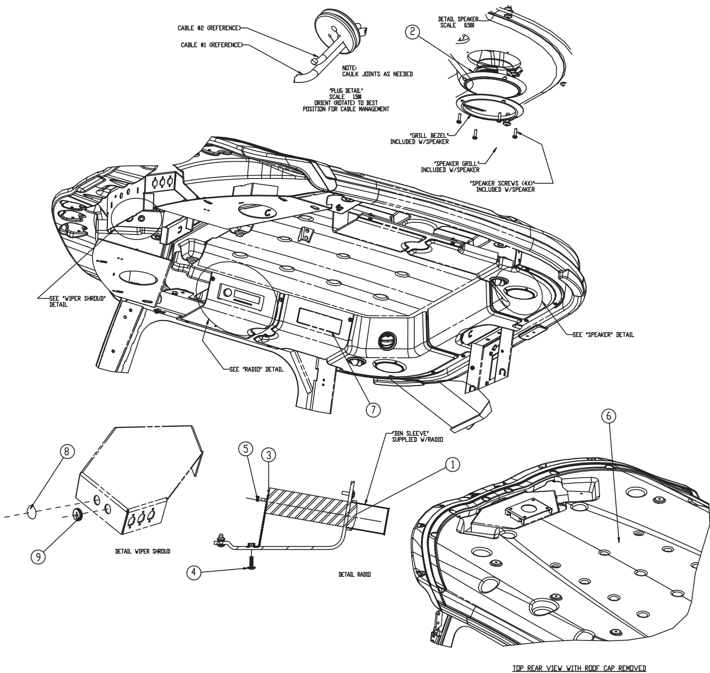
TOP REAR VIEW WITH ROOF CAP REMOVED
