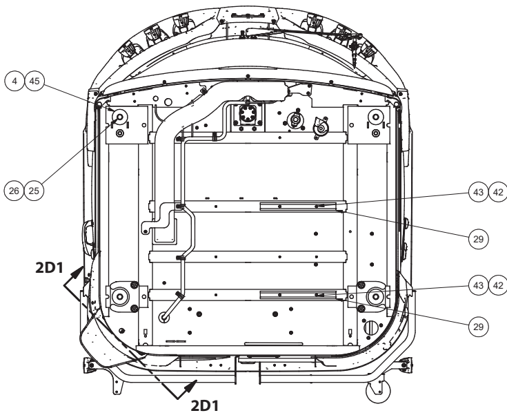
VIEW 1C1-1C1
