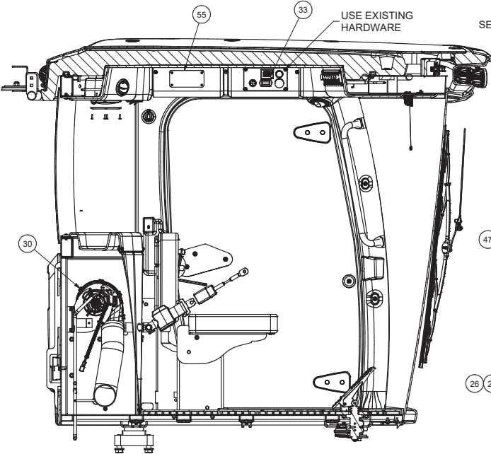
SECTION 2A1-2A1
