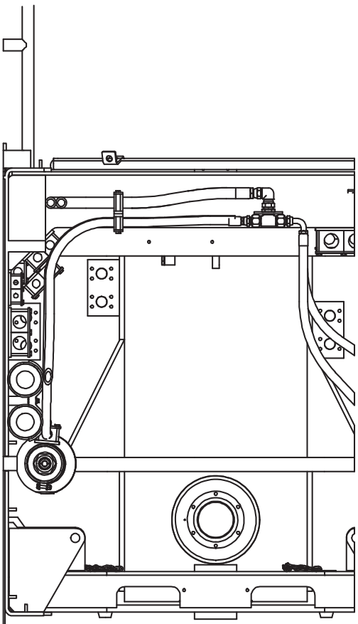
SECTION F-F VIEW ROTATED FOR CLARITY
