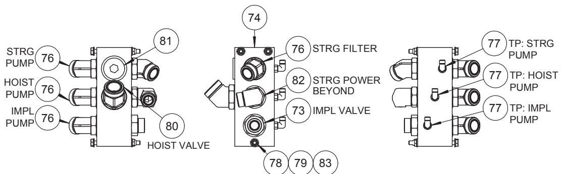
DETAIL 4B4 PRESSURE MANIFOLD
