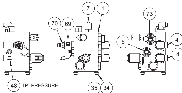
DETAIL 4A4 FAN CONTROL MANIFOLD
