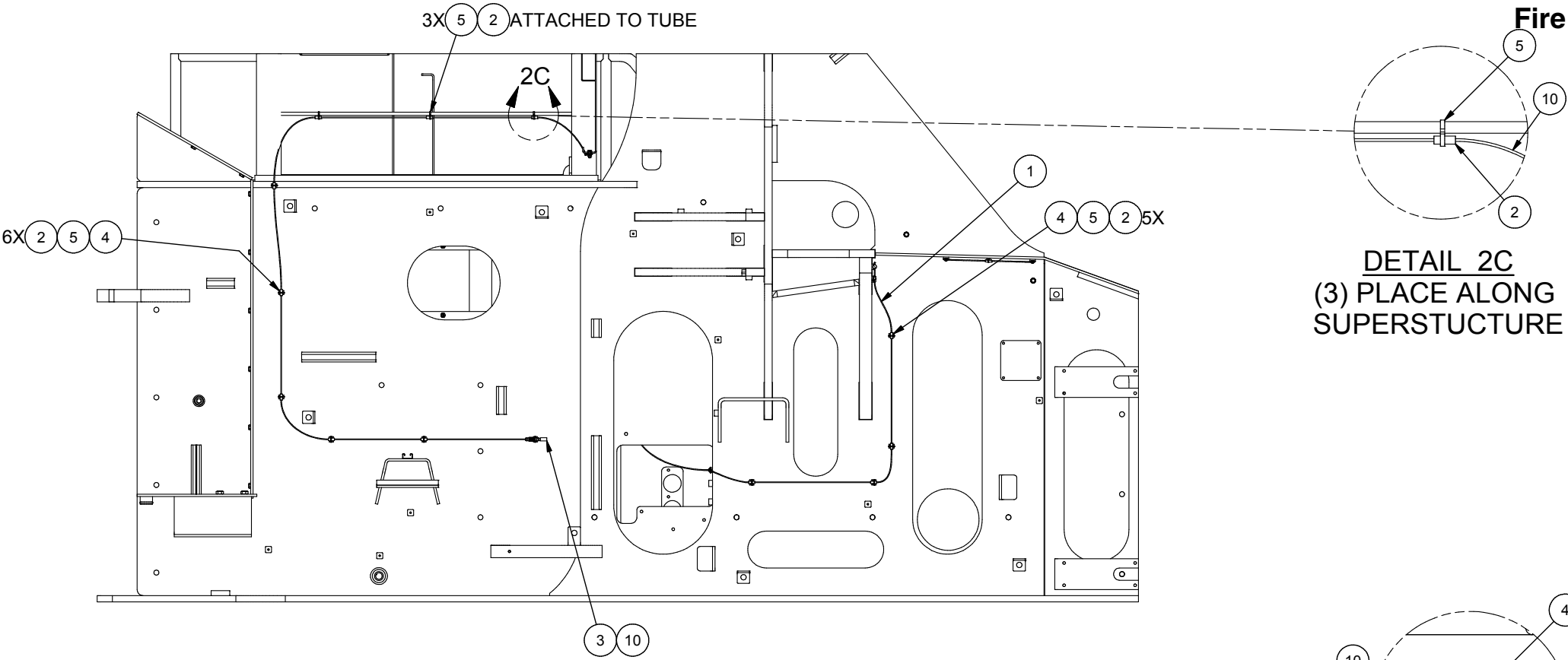
SECTION 2A-2A SOME COMPONENTS NOT SHOWN FOR CLARITY
