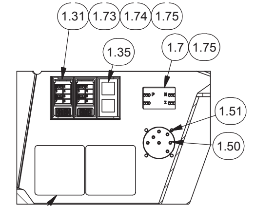
SECTION 3C-3C
