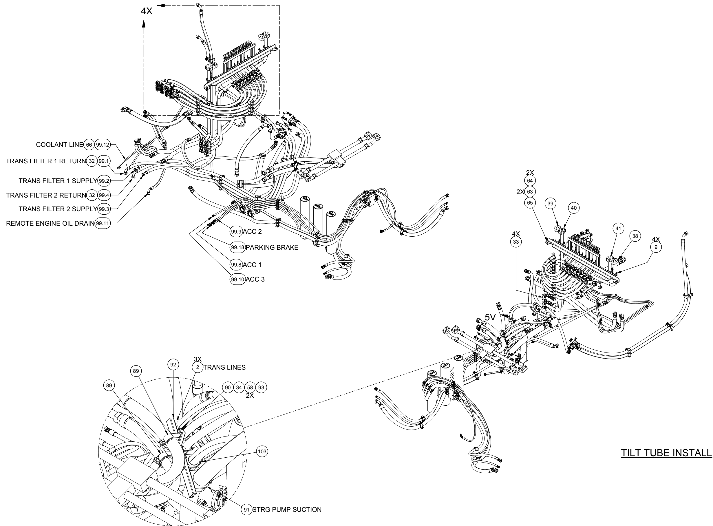
DETAIL 5V TRANSMISSION HOSE TAPER INSTALL
