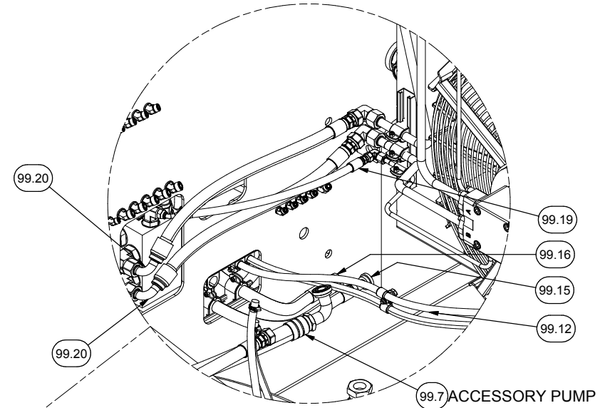
DETAIL 6M HYD COOLING & STRG PLUMBING
