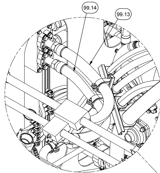
DETAIL 6K HOIST PLUMBING
