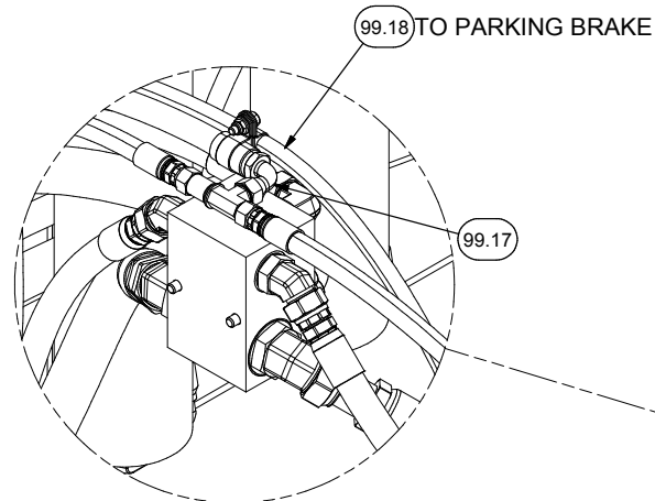
DETAIL 6N BRAKE COOLING PLUMBING
