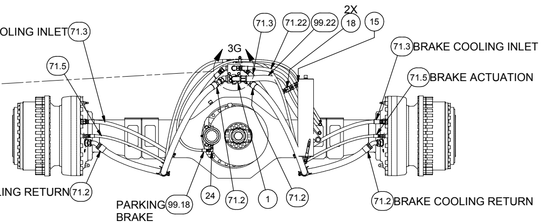
SECTION 3H-3H BRAKE HYD INSTALL
