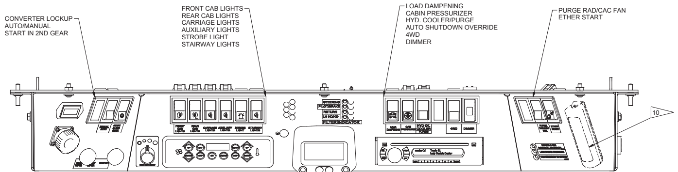
AUTOMATIC TRANSMISSION CONSOLE L60 LAYOUT
