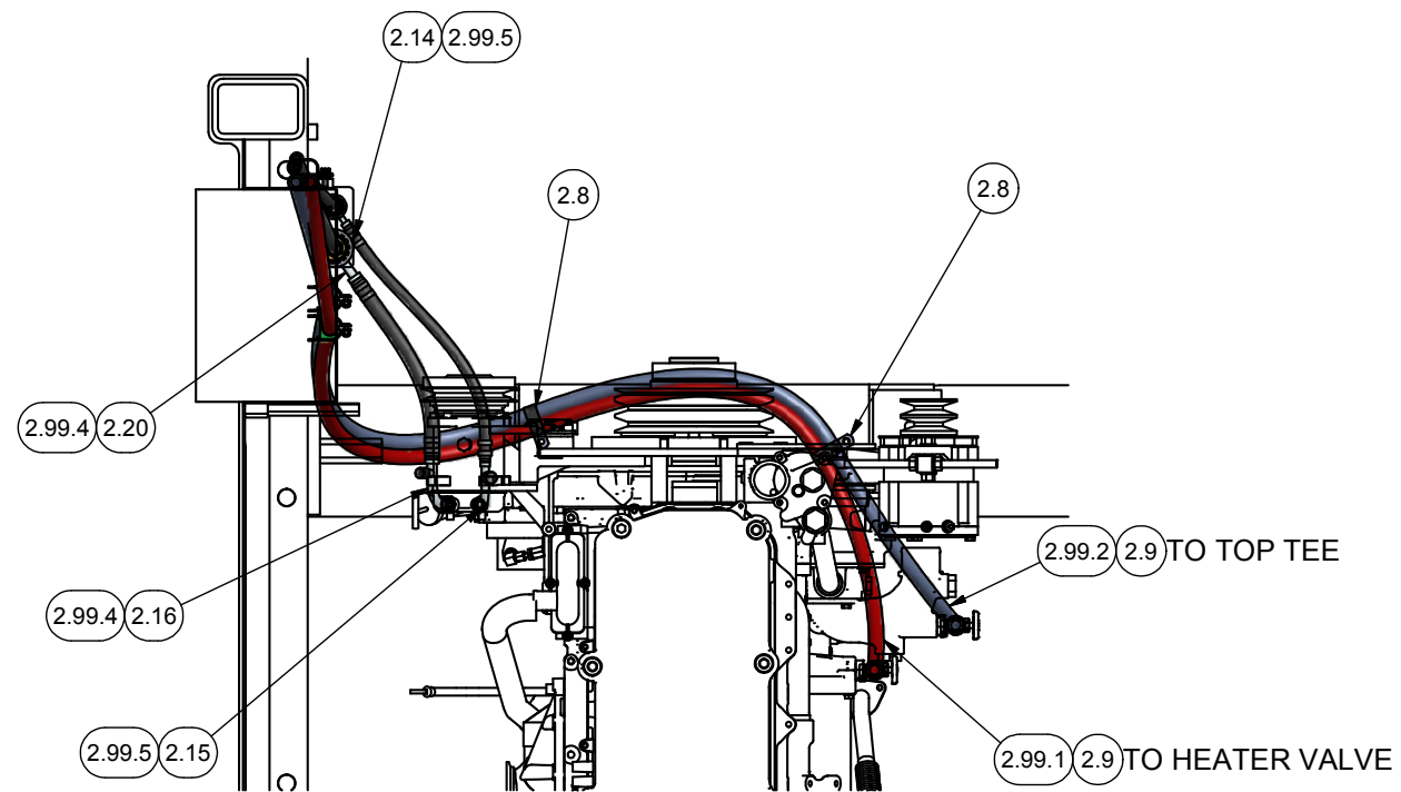
SECTION 4N-4N
