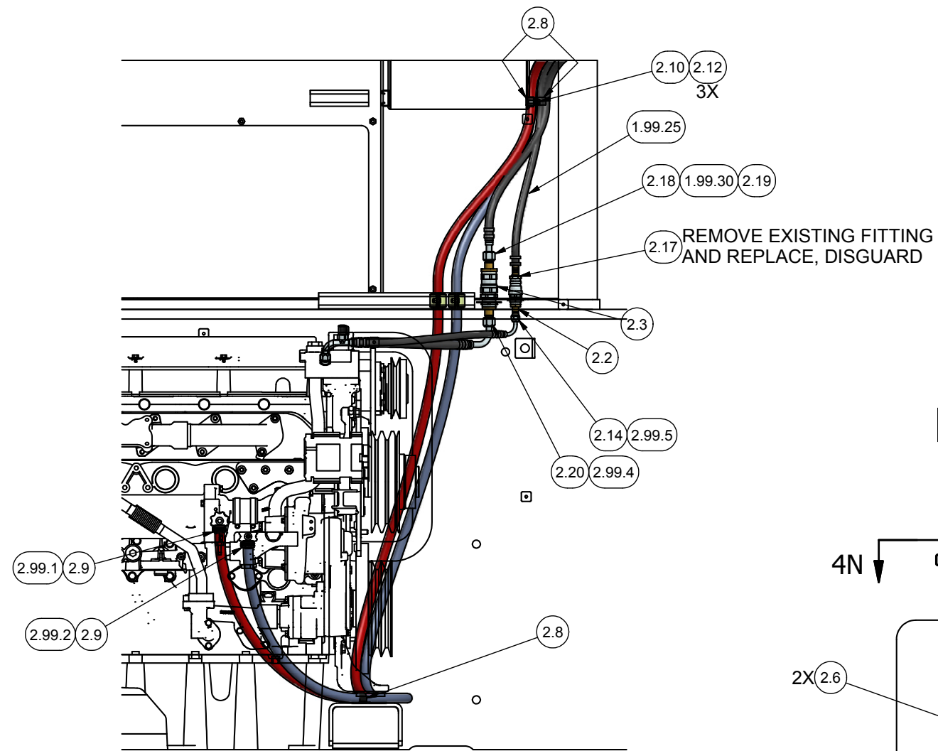
SECTION 4P-4P
