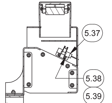
SECTION 10S-10S
