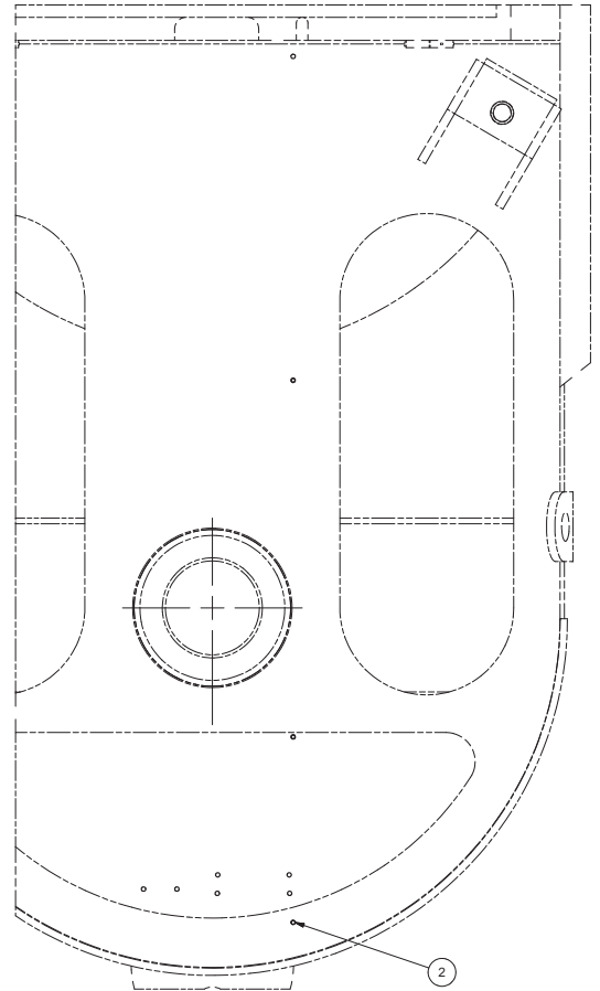
BALLAST COVER
