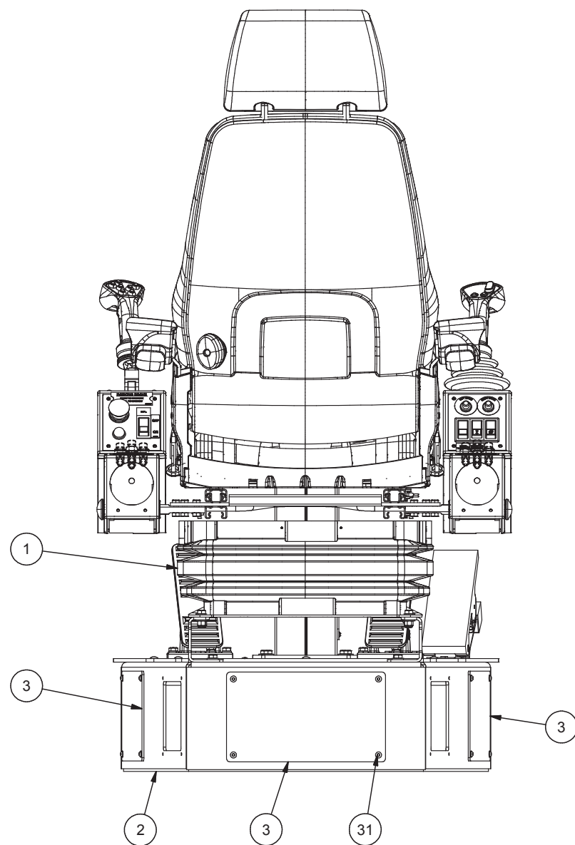
SECTION A1-A1
