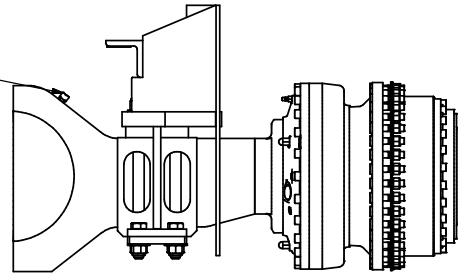
VIEW D-D REAR AXLE BOTH SIDES
