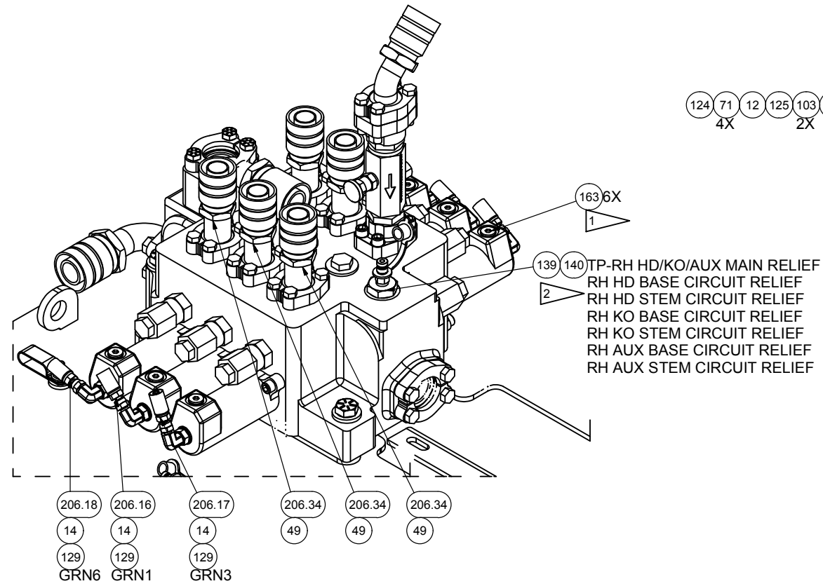
RH IMPLEMENT - FRONT
