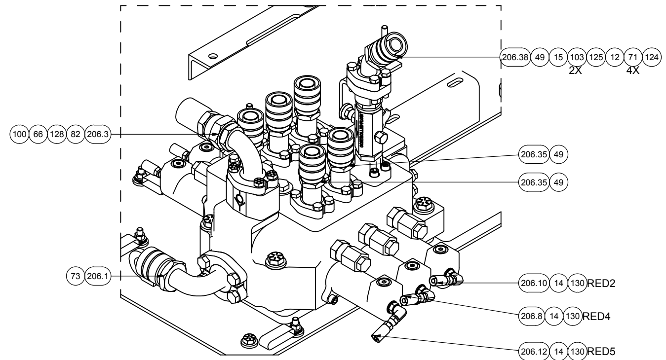
LH IMPLEMENT - REAR
