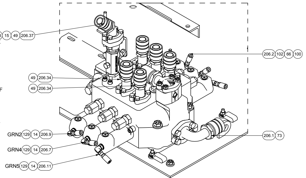
RH IMPLEMENT - REAR
